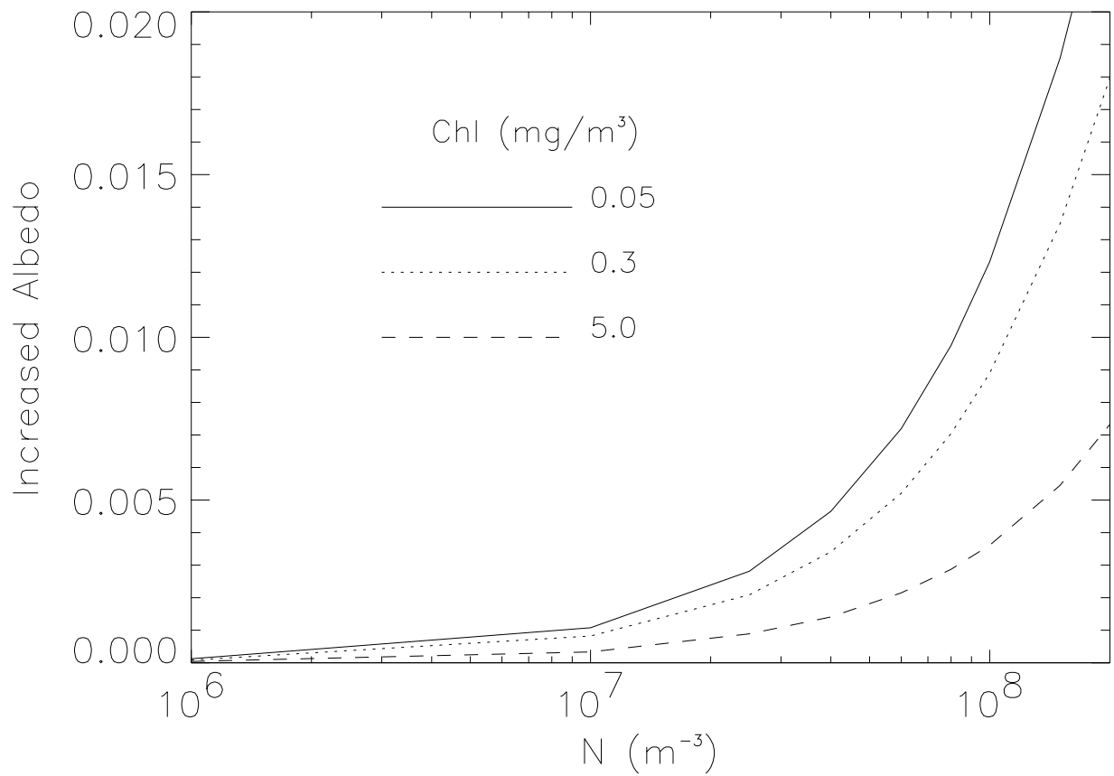
Fig. 11, The change in broad-band albedo as a function of bubble number density for three different Chl concentrations and solar zenith angle of 60°.
