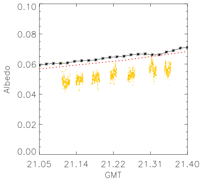
Model–Observation Comparison for CLAMS on 8/1,2001.
