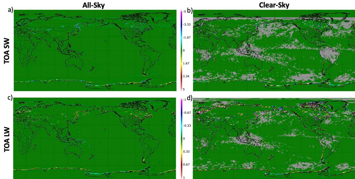
Figure 2-1. Differences in SSF1deg Ed4A monthly mean TOA fluxes ( \text{W m}^{-2} ) in January 2021 due to the change in the supplemental snow/ice dataset.
