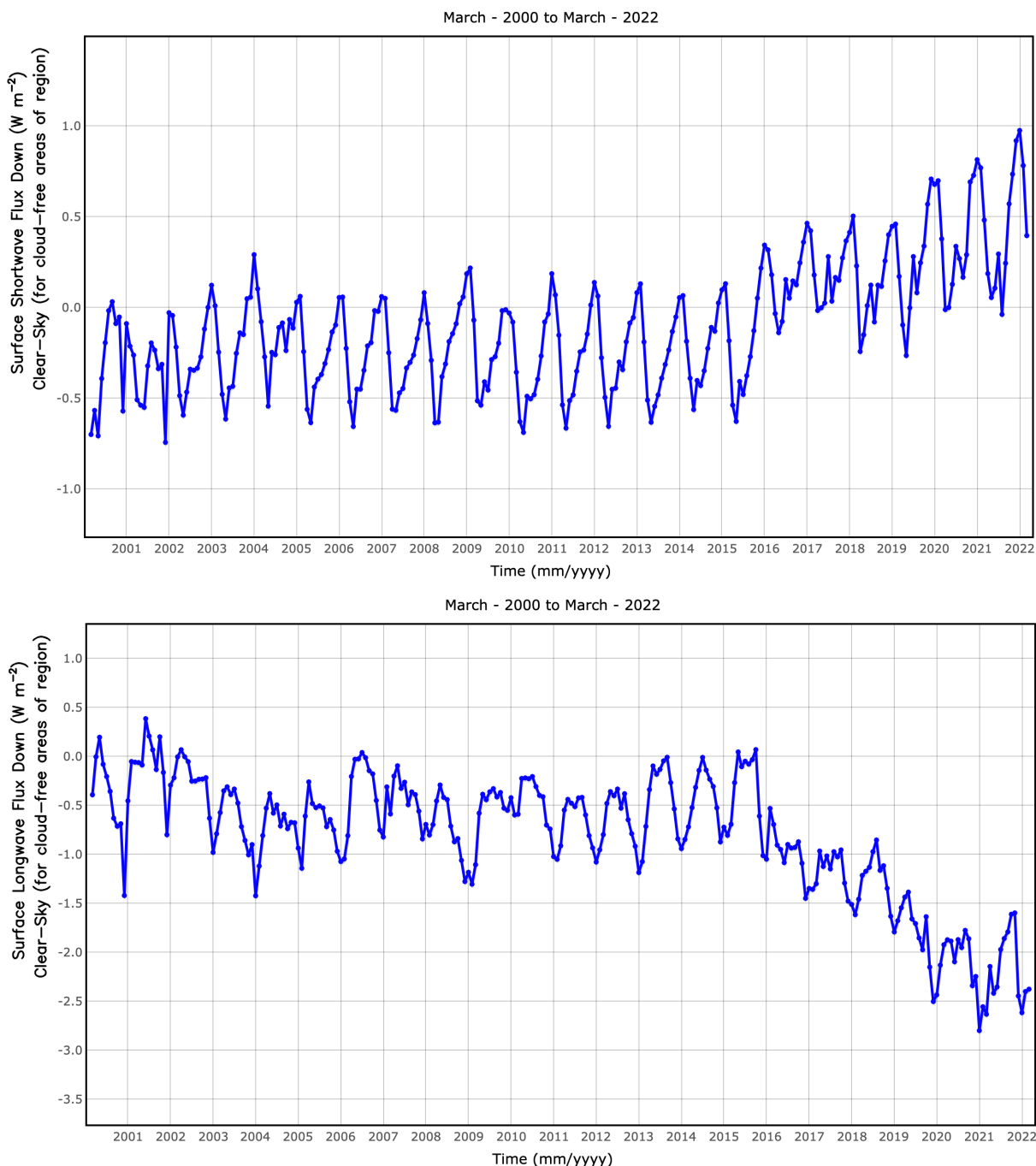
Figure 2-2. Time series of global mean (top) downward shortwave and (bottom) downward longwave flux differences (Ed4.1 minus Ed4.2). Larger difference after 2016 is due to cloud properties and after November 2019 is caused by the drift of GEOS-5.4.1 temperature and humidity used for computing Ed4.1 fluxes (Section 2.1 in EBAF Ed4.1 Data Quality Summary ).
