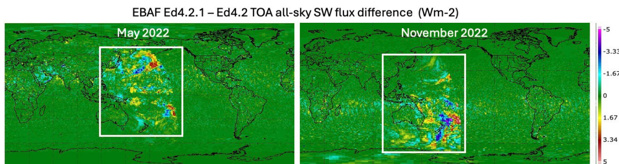
Figure 4-2. The EBAF Ed4.2.1 minus Ed4.2 TOA all-sky SW flux difference in Wm^{-2} shows the impact (denoted by the white box near the dateline) of not using the first day of the following calendar month in the EBAF Ed4.2 product. The EBAF Ed4.2.1 utilized the first day of the following month to compute the regional monthly all-sky SW flux.
