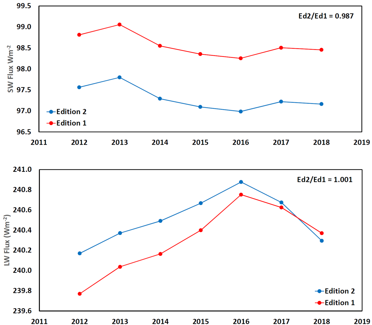
Figure 1. Time series comparisons of global annual mean NPP ES9 all-sky fluxes
