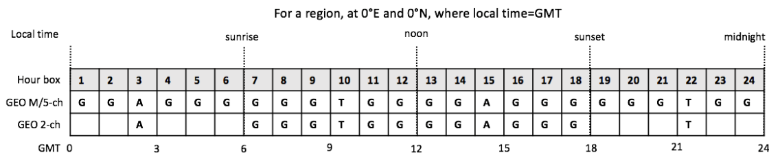
Figure 1-4. A hypothetical 1°-region located at 0° longitude and the equator, where the GMT and local time are identical, monthly GMT 1-hourly distribution of Terra-MODIS, Aqua-MODIS, and GEO cloud retrieval inputs. The GEO 5-ch refers to the 2 nd and 3 rd generation GEO satellites, whereas the GEO 2-ch refers to the 1 st generation GEO satellites shown in Figure 1-2 .
